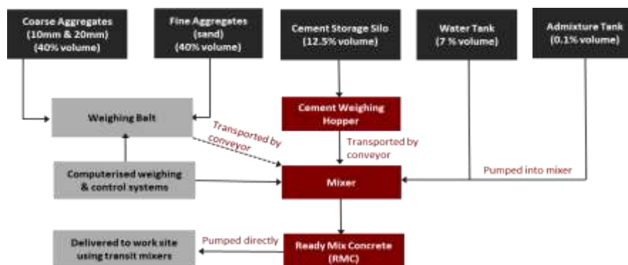
Ready Mix Concrete Production Process Flow Chart
